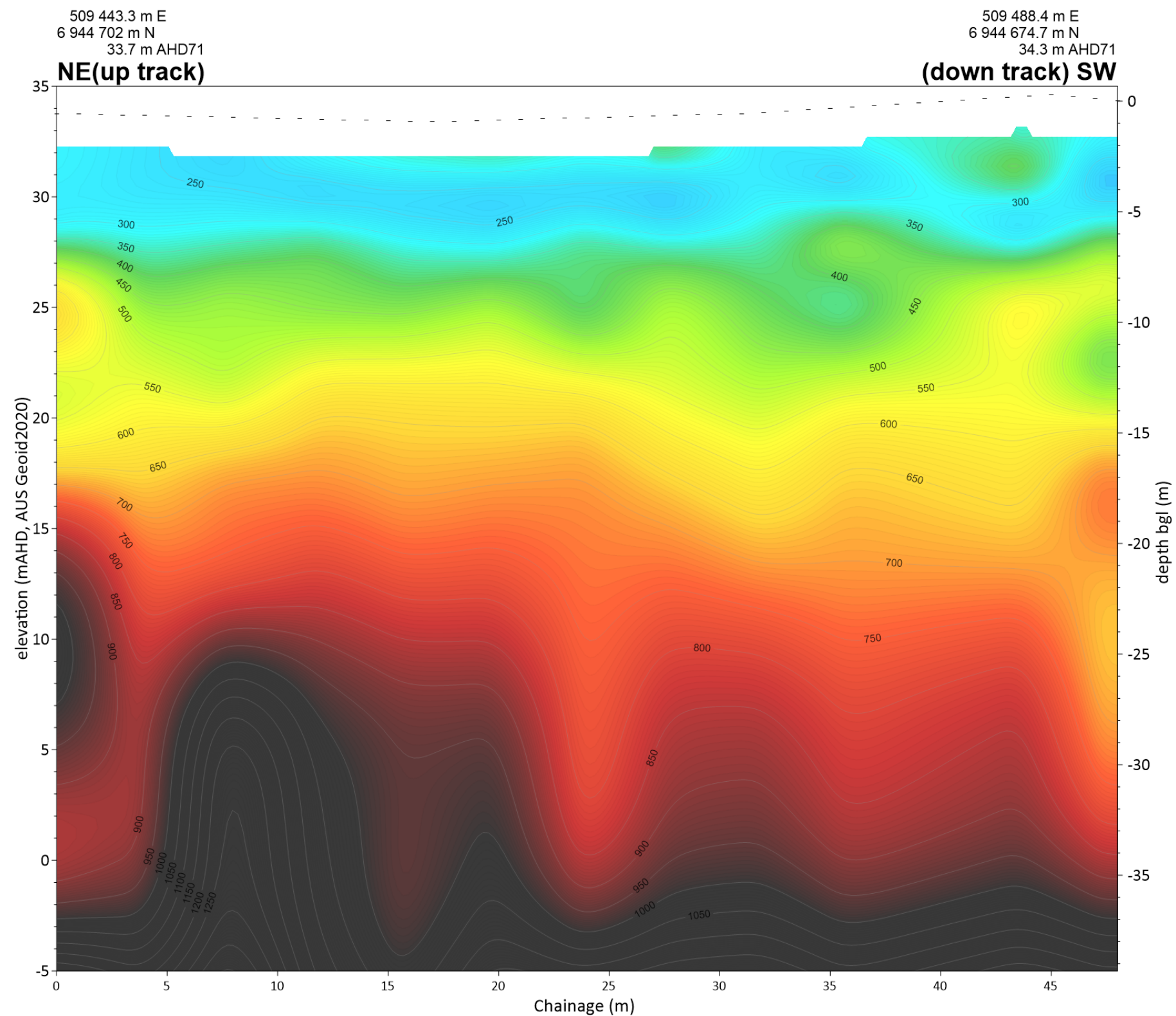
Seismic Line MASW AU-GP 111
